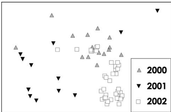
Figure 2. MDS plots for ARISA profiles collected from Crystal Bog over 3 years. Samples collected in 2000 are represented by gray triangles, 2001 samples are black triangles, and 2002 samples are white squares. Stress = 0.15. In order to better visualize the variability among ARISA profiles, the profile generated from the 28 June 2000 sample was omitted from this ordination.
